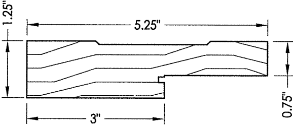
2 WOOD JAMB (SIDELITE)
