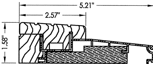
15 INSWING THRESHOLD WORLDWIDE
