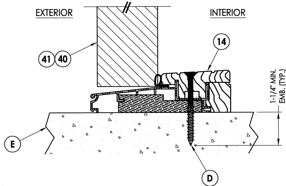
1 VERTICAL CROSS SECTION 10 Outswing
