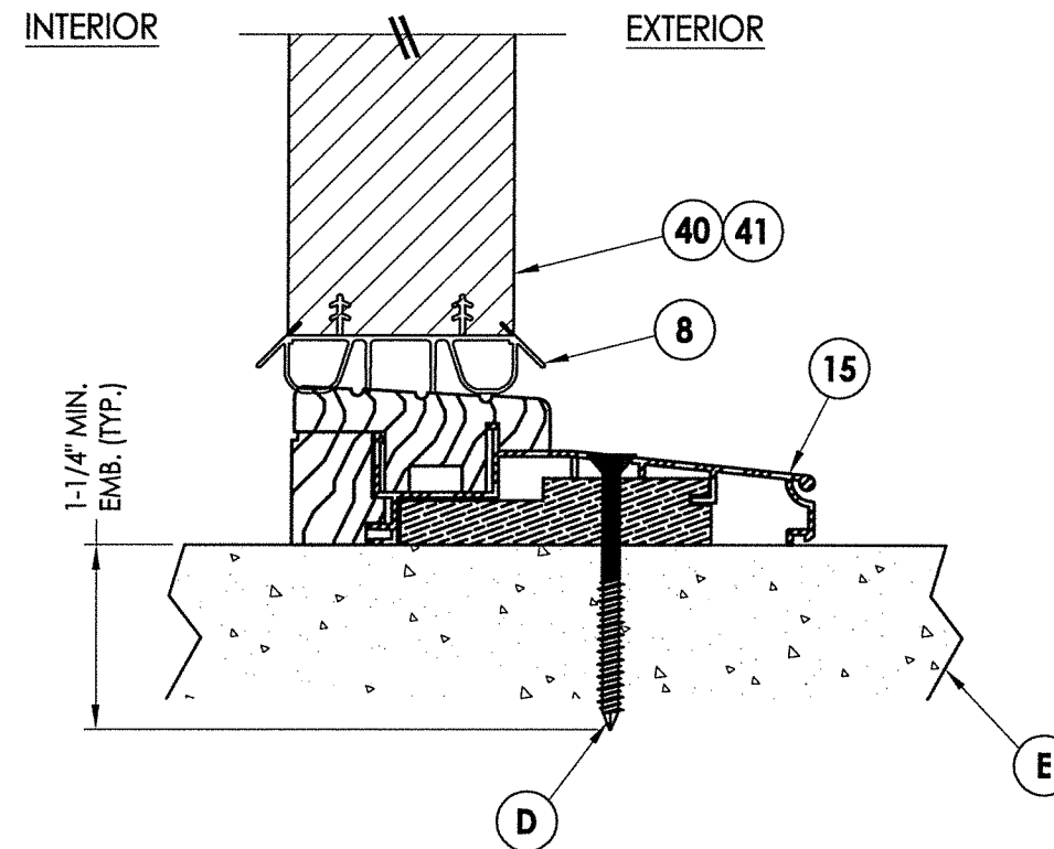
2 VERTICAL CROSS SECTION 10 Inswing
