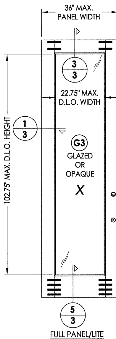
41 WOOD DOOR PANEL (3'-0") Glazed or Opaque
